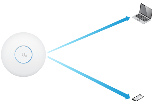
MU-MIMO with 3x3 and 1x1 clients: The UniFi AC SHD AP communicates with one 3x3 client and one 1x1 client at a time.
